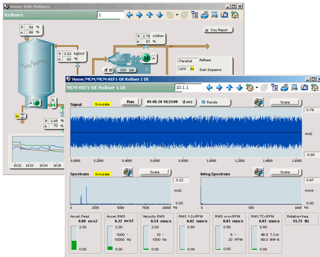
The new user interface combines machine vibration data with process information
